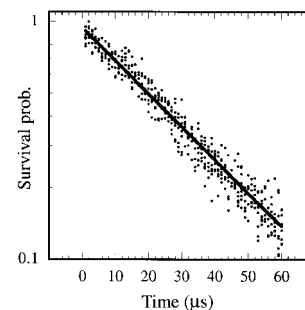
Figure 2 Typical example of experimentally measured survival probability for a small acceleration of 1,200 \text{ ms}^{-2} , a large acceleration of 4,500 \text{ ms}^{-2} , and V_0/\hbar = 50 kHz as a function of the duration of the large acceleration. Note that the vertical axis is logarithmic. The solid line is a fit to an exponential.
