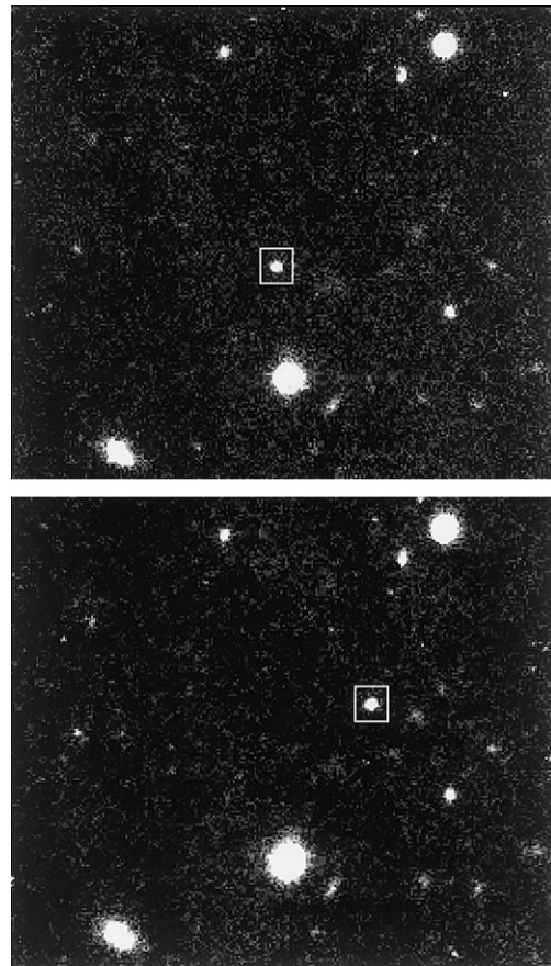
Figure 1 Object 1996TL 66 imaged on UT 1996 October 15 at 07:14 (top panel) and 12:41 (bottom panel). The field shown has north to the bottom, east to the left. Note the relative motion westward against the fixed stars. The field of view is 1.6 \times 1.4 arcmin, representing 0.7% of the total area imaged by the 8K CCD mosaic. The integration time was 600 s through a broadband (5,000–7,000 Å) filter.
