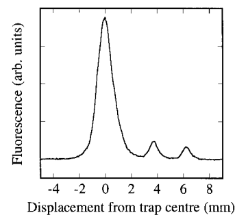
Figure 1 Distribution of atoms after exposure to a three-stage accelerating standing wave for V_0/\hbar = 80 kHz. A small acceleration of 1,500 \text{ ms}^{-2} was first imposed to trap atoms and separate them from the rest of the distribution. A large acceleration of 7,000 \text{ ms}^{-2} was then turned on for a duration of 34 \mu\text{s} . During this stage atoms tunnel from the trapped state, and are lost to the accelerating potential. Finally the same small acceleration was imposed to separate the atoms that have survived from those that have tunneled out. The duration of the three-step process is 1.5 ms, and the total switching time between the three stages is under 500 ns. A free drift of 3 ms allowed the surviving atoms to separate spatially from the main distribution.
