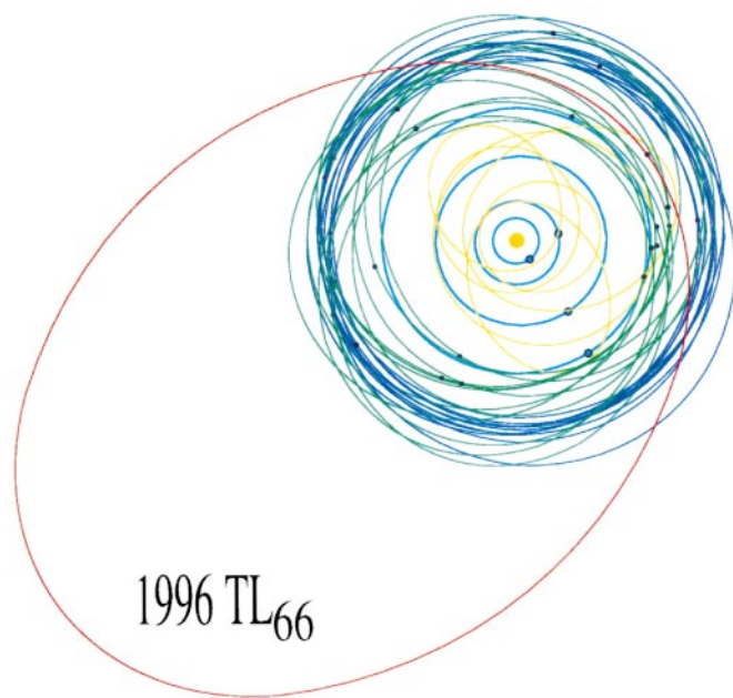
Figure 2 Planar view of the outer Solar System. The four light-blue, nearly concentric orbits are those of the giant planets. The dense band of orbits refers to the best observed Kuiper-belt objects (including Pluto), while the six yellow inner orbits refer to the Centaurs. The large, eccentric orbit of 1996TL 66 extends far beyond the previously known Kuiper belt.
