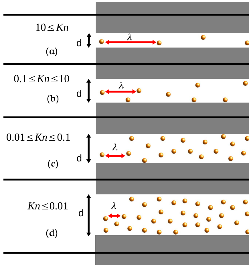
Figure 11. The F diagram shows how the different gas transport processes should evolve as the comet moves from the Oort cloud to the inner solar system, going from high K_n numbers ( K_n = \lambda/d , where \lambda is the mean free path and d is the pore size) to low K_n numbers and changing continuously over a wide range. Flow regimes evolve from Knudsen free diffusion (a), followed by a transition regime (b) that turns into a slip regime (c) that leads to a viscous continuum regime (d). Figure modified from Moghaddam & Jamiolahmady (2016) and https://tinyurl.com/y3xyj9ss .
