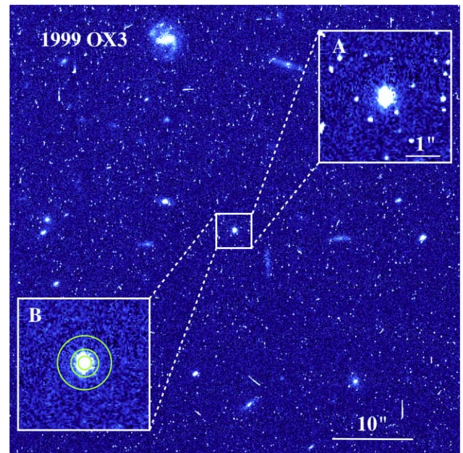
Figure 4. Single 300 s integration HST image of 1999 OX3 at r_{\text{H}} = 18.5 au, shown with a logarithmic stretch between data numbers -0.08 and 0.15 . Panel (A) is a zoomed-in box to show the immediate vicinity of the Centaur. Panel (B) shows the same region as panel (A), cleaned of cosmic rays, and with green circles marking the 0''.2 , 0''.4 , and 0''.8 radius (corresponding to 5, 10, and 20 pixels) photometry apertures.
