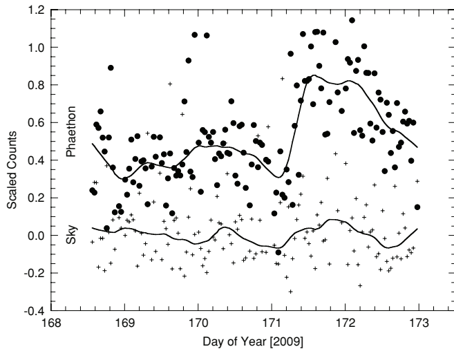
Figure 4. Sky-subtracted data number counts for Phaethon and for a sample patch of sky displaced from Phaethon by 5 pixels (350 arcsec) East and 5 pixels South. The photometry aperture for both Phaethon and the sky was a box of 3 \times 3 pixels while the background was computed from the median of the pixels within a surrounding aperture 5 \times 5 pixels.
