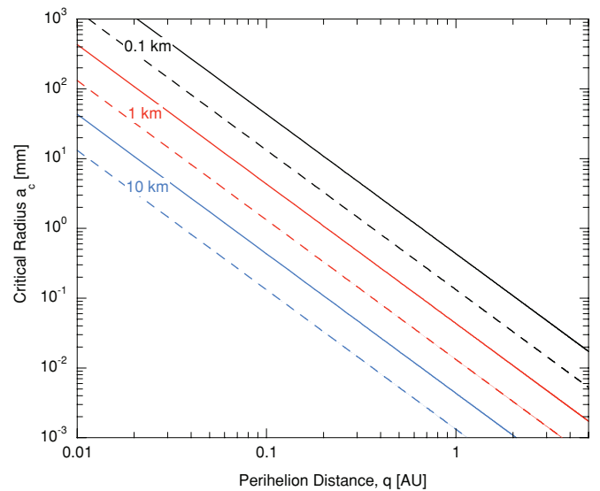
Figure 8. Critical dust radius for radiation pressure sweeping as a function of perihelion distance. Black, red, and blue lines correspond to asteroid radii r_e = 0.1, 1 and 10 km, respectively. Solid lines are for body axis ratios f = 1.4 , dashed lines are for spherical bodies, f = 1 . All other parameters in Equation (6) are the same as those for Phaethon.
