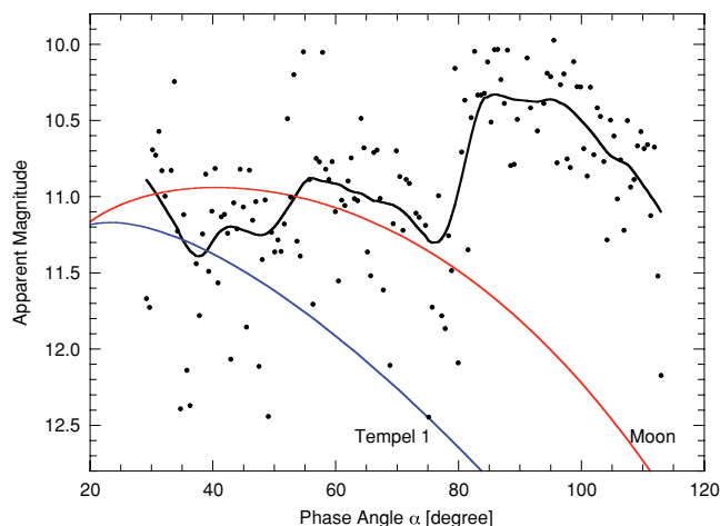
Figure 6. Apparent magnitude vs. phase angle for Phaethon (black points). The black line shows a running box mean capturing 15% of the data. Red and blue curves show the brightness variation of hypothetical bodies at the position of Phaethon and having phase functions as measured for the Moon (red) and the nucleus of comet P/Tempel 1 (blue). The latter two curves have been arbitrarily shifted in the vertical direction in order to facilitate easy comparison with the data.
