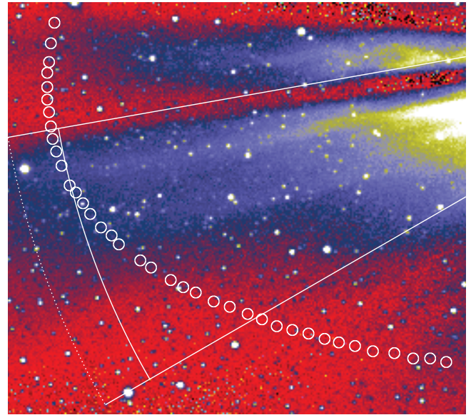
Figure 1. Trajectory of 3200 Phaethon in the field of STEREO camera HI-1A. The coronal image was taken at UT 2009 June 20 08h 49m. Solid arc has radius equal to Phaethon's 0.14 AU perihelion distance and the segment angle of 20^\circ is chosen to highlight the streamer rooted at position angle 110^\circ . Ecliptic north is to the top and east to the left of this 5.0 \times 4.5 degree wide portion of the field of view. The Sun is off to the right.
