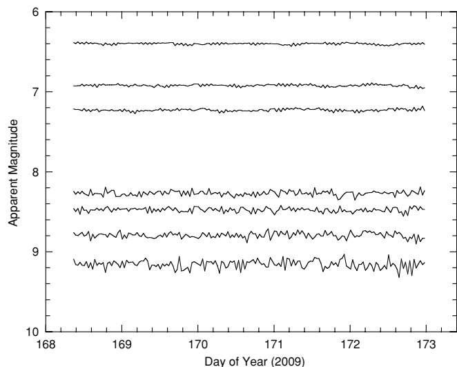
Figure 2. Sample photometry of field stars (numbered) extracted from near the path of 3200 Phaethon, plotted as a function of time. The photometric stability of the system is demonstrated.
