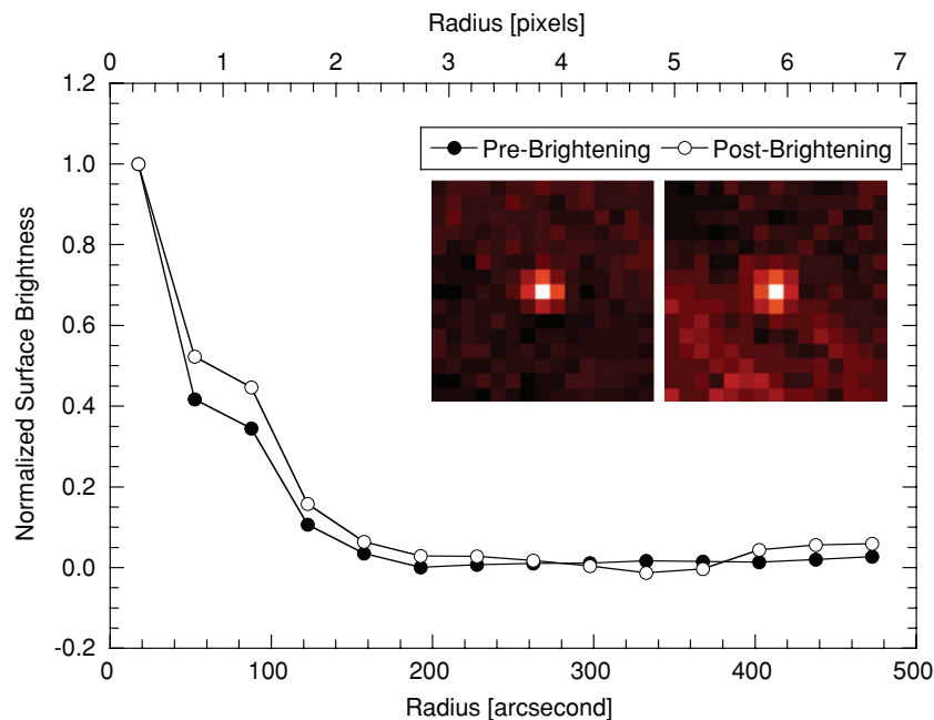
Figure 5. Surface brightness profiles of Phaethon pre-brightening (filled circles) and post-brightening (empty circles), computed as described in the text. The upper and lower axes show the radius in pixels and arcseconds, respectively. Both profiles have been normalized to unity in the central pixel. Inset figures show (left) the pre-brightening and (right) post-brightening images used to determine the profiles.
