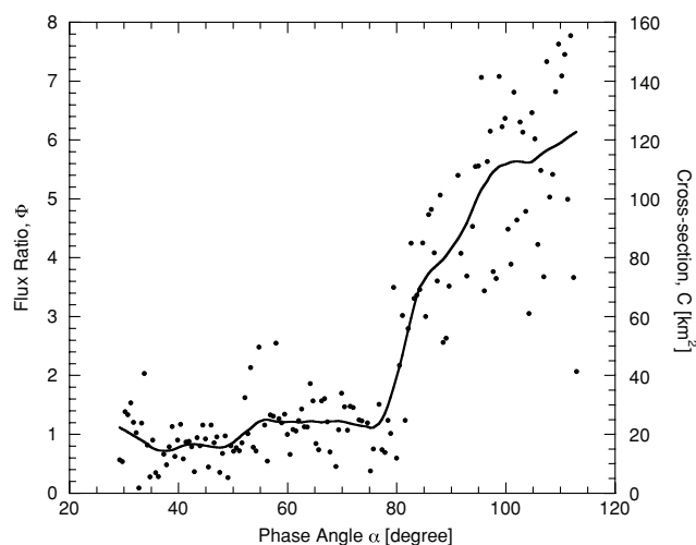
Figure 7. Plot of \Phi , the ratio of the light from Phaethon to the light from the Moon as a function of phase angle, \alpha , normalized to \Phi = 1 in the range 30^\circ < \alpha < 80^\circ . The right-hand axis shows the effective cross section in square kilometers, assuming that \Phi = 1 corresponds to C = 20 \text{ km}^2 .
