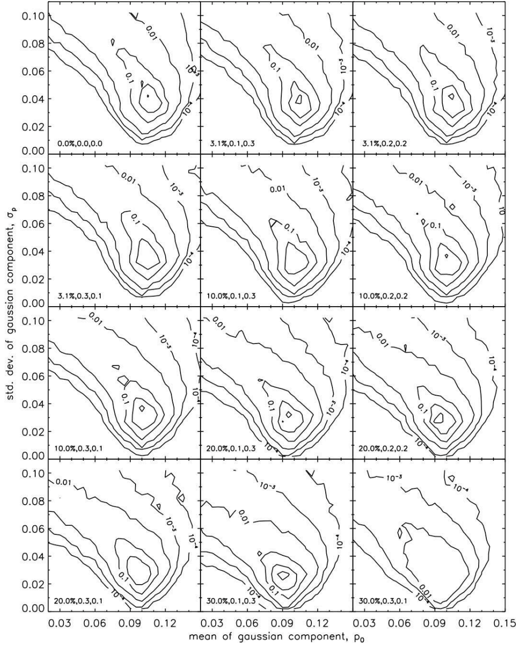
Fig. 5.— Contour plots of the probability that the observed D -vs- p distribution seen in Fig. 1 is drawn from the same distribution as that based on the simulations using the five-parameter model described in §4.2. Each panel represents different values of f_h , p_l , and p_w ; the values are written in the lower left. Contours correspond to probabilities of 10^{-4} (outermost contour), 10^{-3} , 0.01, 0.1, 0.3, and 0.5.
