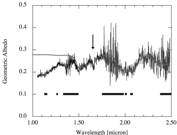
Fig. 11.— Reflection spectrum of KBO (50000) Quaoar in the near infrared, showing broad bands due to water at 1.5 \mu\text{m} and 2.0 \mu\text{m} , and a narrower feature at 1.65 \mu\text{m} that is specifically due to crystalline water ice (arrow). The smooth line is a water ice spectrum that is over-plotted (but not fitted) to the astronomical data. Horizontal bars mark wavelengths at which the Earth’s atmosphere absorbs. From Jewitt and Luu (2004).
