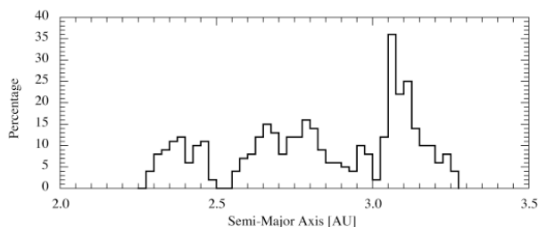
Fig. 6.— Fraction of asteroids (of all spectral types) showing the 0.7 \mu m band attributed to the Fe 2+ \rightarrow Fe 3+ transition in hydrated material. Given that the 0.7 \mu m band is a proxy for OH, the figure may show the distribution of water across the main-belt. Replotted from Carvano et al. (2003).
