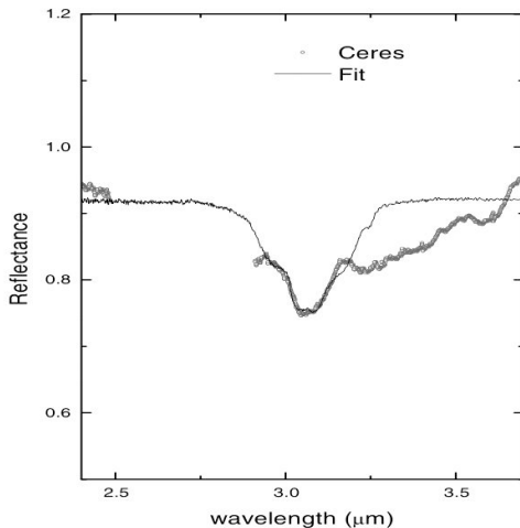
Fig. 7.— Spectrum of asteroid 1 Ceres showing the 3.06 \mu\text{m} absorption band attributed to crystalline water ice. The thin line is a model fit to the data. An additional absorber is required to match the data at wavelengths longer than 3.15 \mu\text{m} . From Vernazza et al. (2005)
