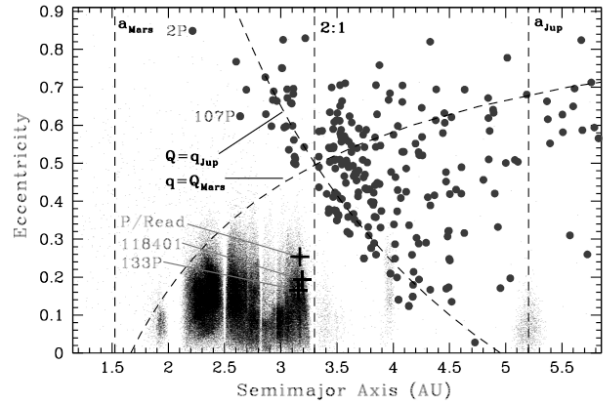
Fig. 9.— Semimajor axis vs. orbital eccentricity showing main-belt asteroids (small dots), active Jupiter family comets (large filled circles) and the three established main-belt comets (plus signs, labeled). Vertical dashed lines at 1.5 AU and 5.2 AU mark the semimajor axes of the orbits of Mars and Jupiter, respectively, while the 2:1 mean-motion resonance with Jupiter (which practically defines the outer edge of the main-belt, is shown at 3.3 AU. Curved dashed lines show the loci of orbits which have perihelia inside Mars’ orbit or aphelia outside Jupiter’s. Objects above these lines are Mars and/or Jupiter crossing. The MBCs are far below both lines with the main-belt asteroids and distinct from the Jupiter family comets. Figure from Hsieh and Jewitt (2006).
