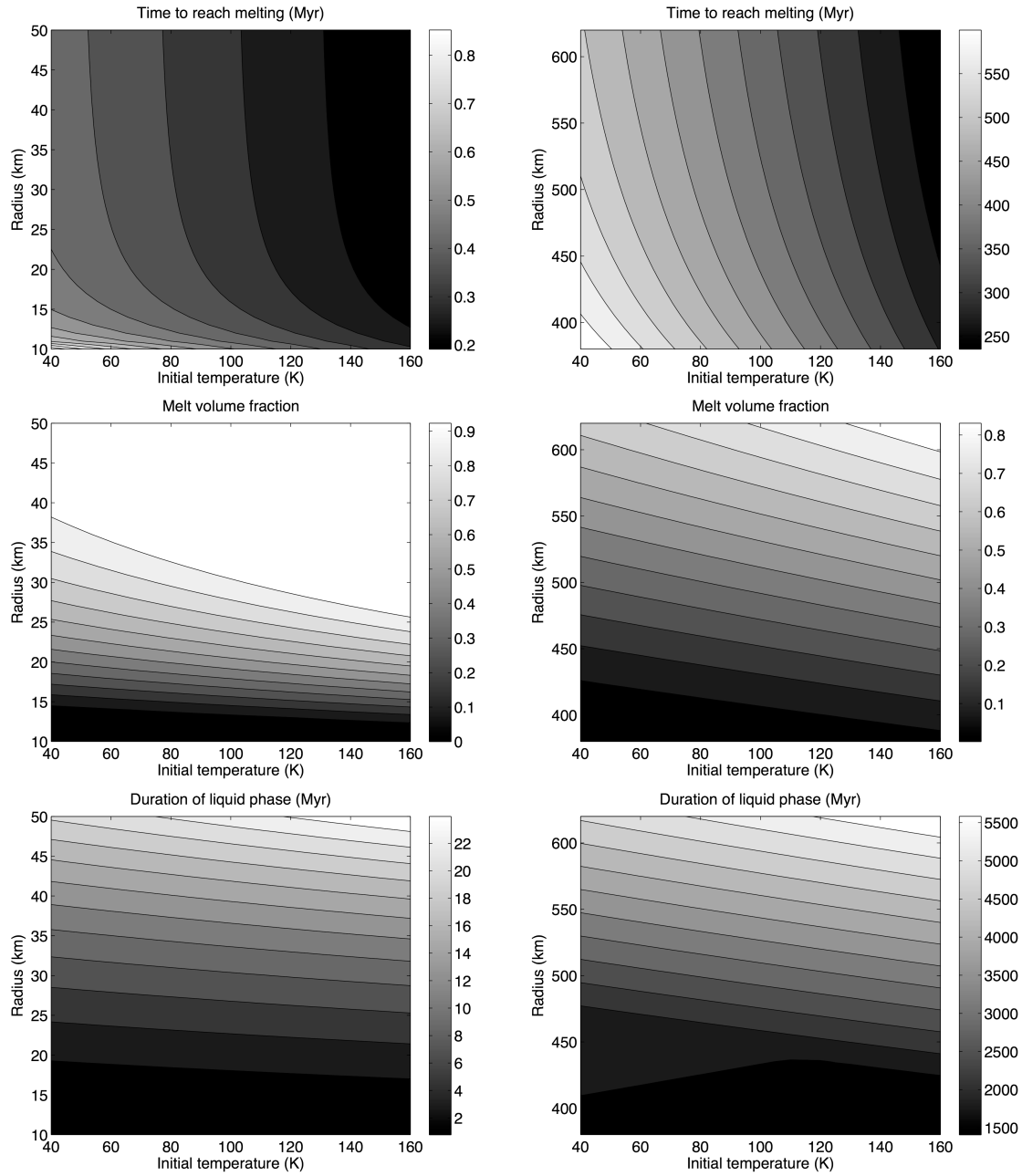
Fig. 13.— Models for the thermal evolution of small bodies heated by radioactive decay as a function of their radius and initial temperature assuming a 1:1 ice: rock mass ratio. Left and right columns show models heated by the decay of ^{26}\text{Al} and ^{40}\text{K} , respectively (see text). At the top is shown the time to reach the water ice melting point, in the middle is the fractional melt volume while at the bottom is the duration of the liquid phase.
