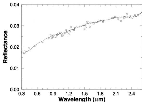
Fig. 10.— A comparison of the reflectance spectra of Tagish Lake (line) with the D-type asteroid (368) Haidea (points). Figure courtesy of Hiroi et al. (2001) .
