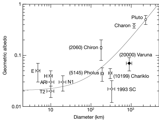
Figure 2 Well determined albedos and diameters of outer Solar System objects. The nuclei of short-period comets are: E, P/Encke 6 ; AR, P/Arend-Rigaux 5 ; T2, P/Tempel 2 (ref. 4); N1, P/Neujmin 1 (ref. 3); and H, P/Halley 22 . Other objects include centaurs (2060) Chiron 23 , (5145) Pholus 24 and (10199) Chariklo 13 , and Pluto and Charon 25 . The albedo of Charon should be considered an upper limit, owing to near-nucleus dust coma contamination. A 2.7 \sigma confidence limit to the 90- \mu m flux from the Infrared Space Observatory on 1993 SC was used to obtain estimates for the diameter (328 +58 -66 km) and albedo (0.022 +0.013 -0.006 ), while object 1996 TL66 was not detected at its expected position 14 . Thermal observations of KBOs will be an important objective of NASA's upcoming SIRTf satellite. The solid line shows the linear correlation between albedo and diameter. The linear correlation coefficient for the objects is 0.92, and the probability that this or a larger correlation might be obtained by chance from uncorrelated data is P(0.92, 12) < 10^{-4} . Removal of Pluto from the plot reduces the correlation coefficient to 0.79, for which P(0.79, 11) = 0.004 , which is statistically insignificant (3 \sigma corresponds to P = 0.003 ). Plotted error bars are all 1 \sigma . P(x, y) notation indicates the correlation coefficient, x , and the number of data points, y .
