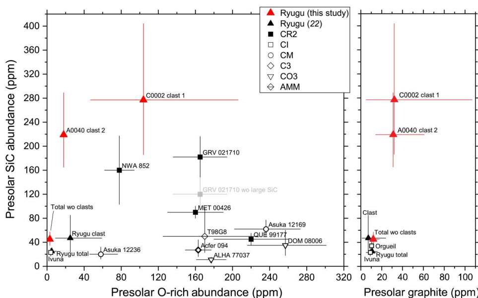
Fig. 5. Abundances of presolar grains in Ryugu, carbonaceous chondrites, and an AMM. Abundances of presolar silicates and oxides (O-rich), SiC, and graphite in clasts 1 and 2 and Ryugu matrix compared to abundances in chondrites of various classes [(9) and references therein (10, 18, 19, 22, 33, 36, 37, 51)] and an AMM (31). The abundances in Ryugu are consistent with CI chondrites except for clasts 1 and 2, which have remarkably high abundances of presolar SiC grains. The presolar silicate abundance in clast 1 is similar to primitive chondrites and not altered CI. Presolar O-rich grain abundances for A0040 clast 2, total Ryugu without clasts, and Ivuna (22) are upper limits. Errors are 1\sigma . wo, without. Not plotted are presolar grain abundances in comet Wild 2 and IDPs. The abundance of O-rich presolar grains in comet Wild 2 samples is 600 to 830 ppm, and the abundance of presolar SiC is 45 ppm (26). Anhydrous IDPs display a wide range of presolar abundances for O-rich grains (20 to 23,080 ppm including 1\sigma errors) and SiC grains (10 to 630 ppm including 1\sigma errors) (21, 27, 34, 35).
