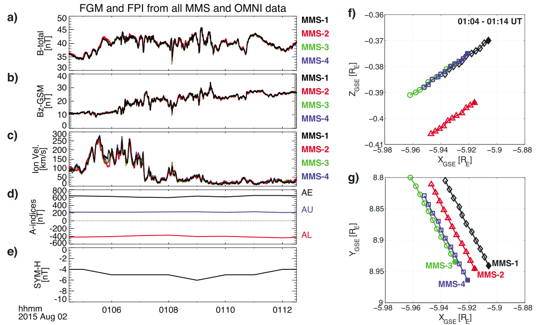
Figure 1. (a–c) Magnetic field magnitudes and the z_{GSM} component from the FGM and partial ion velocity moments from FPI from all four spacecraft, corresponding to different colors as labeled. Note that the ion velocity magnitude is affected by contaminating background after \sim 01:06 UT. (d and e) The AE, AL, AU, and SYM-H indices. (f and g) A zoom-in on the spacecraft locations in the GSE coordinate system in units of Earth radii ( R_E ). Symbols (diamond, triangle, circle, and square for MMS-1, MMS-2, MMS-3, and MMS-4, respectively) are shown at 1 min intervals from 01:04 (solid symbol) to 01:14 UT on 02 August 2015. Figure 1f shows projections onto the x-z plane, while Figure 1g shows projections onto the x-y plane. The colors correspond to those shown in Figures 1a–1c for each spacecraft.
