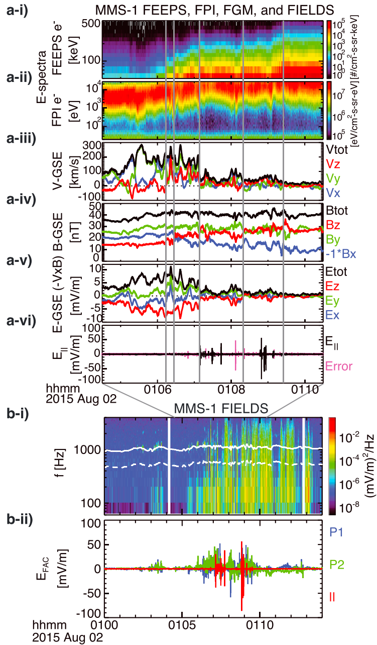
Figure 2. (a-i to a-vi) FEEPS, FPI, and FGM data from MMS-1 during the period of interest. From top to bottom, the panels show FEEPS differential flux energy distributions, with flux in color (log scale) plotted versus energy and time; FPI energy flux distributions in the same format (note different units); ion speed (black) and velocity components (colors); magnetic field magnitude (black) and vector components (colors); electric field magnitude (black) and vector components (colors) calculated using -V \times B ; and the parallel component of the fast survey electric field (black) with an estimate of the error in magenta, which is a weighted average of the axial electric field residuals from the effects of spacecraft charging, a cold plasma wake, and harmonics of the satellite spin tone. For the three vector plots, components are shown in the GSE coordinate system and colors correspond to the directions labeled on the side of the plots. Note that the ion velocity magnitude is affected by contaminating background after \sim 01:06 UT. Note too that for the magnetic field plot, the x component has been multiplied by -1 to limit the y axis range and reveal more detail. The vertical gray lines mark the clearest dipolarization events discussed in the text. (b-i to b-ii) Observations of the electric fields and waves observed by the FIELDS instrument suite on MMS-1. From top to bottom are the electric field power spectral density (in color) frequency spectrogram; electric field vector in field aligned coordinates (FAC) from the fast survey data (128 Hz). The white solid and dashed lines in Figure 2b-i are the electron cyclotron frequency ( f_{ce} ) and 1/2 f_{ce} , respectively. For E_{FAC} , the magnetic field vector ( \mathbf{B} ) corresponding to each electric field vector was used to define “P1” as the component perpendicular to \mathbf{B} and in the spacecraft spin plane, “||” as the component parallel to \mathbf{B} , and “P2” that completes the right-handed system.
