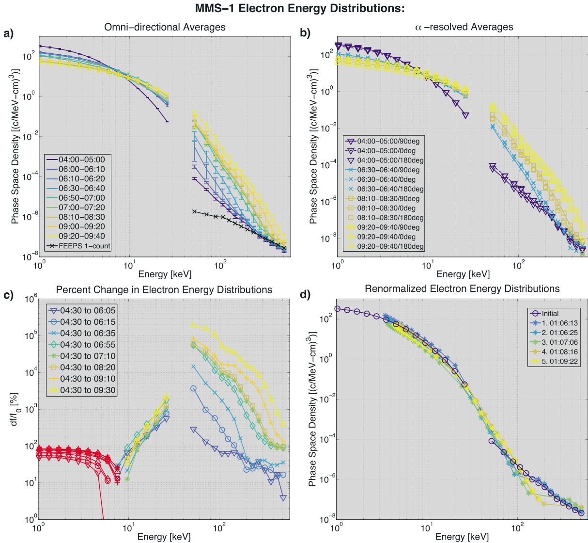
Figure 3. Electron phase space density distributions measured by FPI and FEEPS on MMS-1. (a) Omnidirectional average distributions averaged over the time ranges shown in the legend. Note that the times are listed in minutes and seconds (mm:ss); all of them have the same hour, 01:00 UT. The error bars are \pm 1\sigma from the averaging, and the black line with x marks shows the 1 c/s level for the FEEPS instruments. (b) A subset of the distributions resolved by pitch angle, with those for 90° electrons shown with solid lines and those for 180° and 0° electrons shown with dotted and dashed lines, respectively. Note that distributions from only four of the time periods are shown in Figure 3b. (c) The percent-difference between the initial distribution (01:04:00–01:05:00 UT) and each subsequent distribution (see legend for corresponding times) as a function of energy. The red curves show where the percent difference was negative; these values have been multiplied by -1 to show on the logarithmic scale. (d) The electron distributions from Figure 3a (in corresponding colors) but renormalized using the simple model from equations (1) and (2). The initial distribution is the same as that from 04:00–05:00 in Figure 3a, but the remaining curves, which correspond to the distributions during/after each of the five identified dipolarizations/injections, have been renormalized using the following model parameters: \epsilon_{\min} = [4, 6, 8, 10, 12] keV; \epsilon_{\max} = [150, 200, 320, 500, 600] keV; B_{zf} = [16, 21, 27, 25, 33] nT; B_{zi} = 11 nT. The five values given correspond to each of the distributions from injections 1 to 5, respectively, and these values are a posteriori approximations from the actual MMS observations during this series of events.
