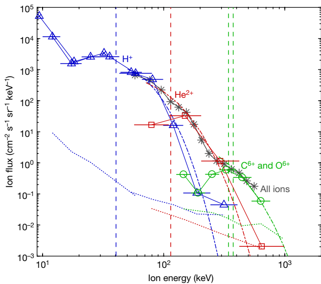
Fig. 4 | Comparing observations and theory. Energy distributions of ions with energies of tens to hundreds of kiloelectronvolts determined from the HPCA, EIS and FEPS instruments on all four MMS spacecraft for the period 05:30:00–05:31:25 UT are shown as solid lines and markers. Data for heavy (CNO branch) and helium ions are shown as green circles and red squares, respectively. Proton data from HPCA are shown as blue triangles around blue crosses; proton data from the EIS energy-by-time-of-flight ( E \times \text{TOF} ) technique are shown as open blue triangles; and proton data from the EIS pulse-height-by-time-of-flight ( \text{PH} \times \text{TOF} ) technique are shown as blue triangles around blue plus signs. On all EIS data points, the solid horizontal lines show the energy range of each channel. The dotted lines show one-count background levels for the EIS data. EIS \text{PH} \times \text{TOF} data have been cross-calibrated to HPCA and E \times \text{TOF} data where there is overlap between those instruments. FEPS data, which do not distinguish between different ion species, are shown as grey lines and asterisks. FEPS data have had a constant cross-calibration factor of two applied to all energy channels. The dashed vertical lines represent E_{\text{max}} from equation (2) in Methods (the maximum energy in a Fermi acceleration trap of size L ) for protons ( \text{H}^+ , blue), \alpha particles ( \text{He}^{2+} , red) and heavy ions ( \text{C}^{6+} and \text{O}^{6+} , green) using a constant in equation (2) in Methods calculated for 40-keV protons (with mass m = 1 and charge q = 1 ). The dash-dotted, exponentially decaying lines show numerical solutions for the high-energy tails of the distributions of protons (blue), \alpha particles (red) and \text{O}^{6+} ions (green) accelerated between the observed HFA and Earth's bow shock, using the Fermi acceleration model derived in Methods.
