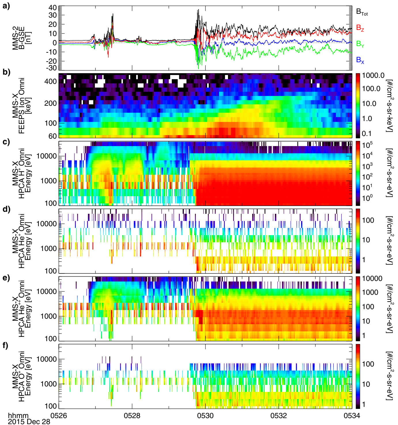
Extended Data Fig. 1 | Solar-wind ion species observed by MMS HPCA. a , Magnetic-field vector and strength from MMS-2. b–f , FEEPS total energetic ion ( b ) and HPCA ion ( c–f ) composition flux energy spectra (omni-directional) combined from all four spacecraft (MMS-X). HPCA observed many fewer \text{He}^+ ion than \text{He}^{2+} ions ( \alpha particles) and no \text{O}^+ ions (all zero counts despite energy channels up to about 38 keV) at E > 10 keV during the observation of the energetic ions between the HFA and the
