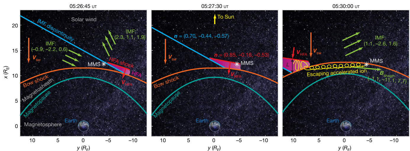
Fig. 3 | Conceptual scenario for the HFA observed by MMS on 28 December 2015. Earth is shown at the origin of three two-dimensional cross-sections (approximately in Earth's equatorial plane; R_E is the radius of Earth), which capture the geometry of the system at 05:26:45 UT, 05:27:30 UT and 05:30:00 UT (left to right). The position of MMS is marked by the white asterisk. Slices of Earth's magnetopause, Earth's bow shock, the IMF discontinuity and the HFA shock are shown in turquoise, orange, blue and red, respectively. Velocity vectors for the solar wind ( V_{sw} ) and the HFA shock ( V_{HFA} ) are also shown. IMF geometries and vectors are shown in green, and the normal vectors of the IMF discontinuity ( \mathbf{n} = (0.70, -0.44, -0.57) ) and the HFA shock ( \mathbf{n} = (0.85, -0.16, -0.53) ) are also labelled. The core of the HFA is shown in magenta. As the IMF discontinuity and HFA convect with the solar wind, they sweep from right to left across the bow shock, as shown here. The HFA grows in time as it sweeps up and concentrates more and more suprathermal ions in the quasi-parallel foreshock that forms on the upstream side (towards the Sun) of the IMF discontinuity. In the solar-wind rest frame, Earth's bow shock is moving towards the Sun at V_{sw} (orange velocity vector) and is
