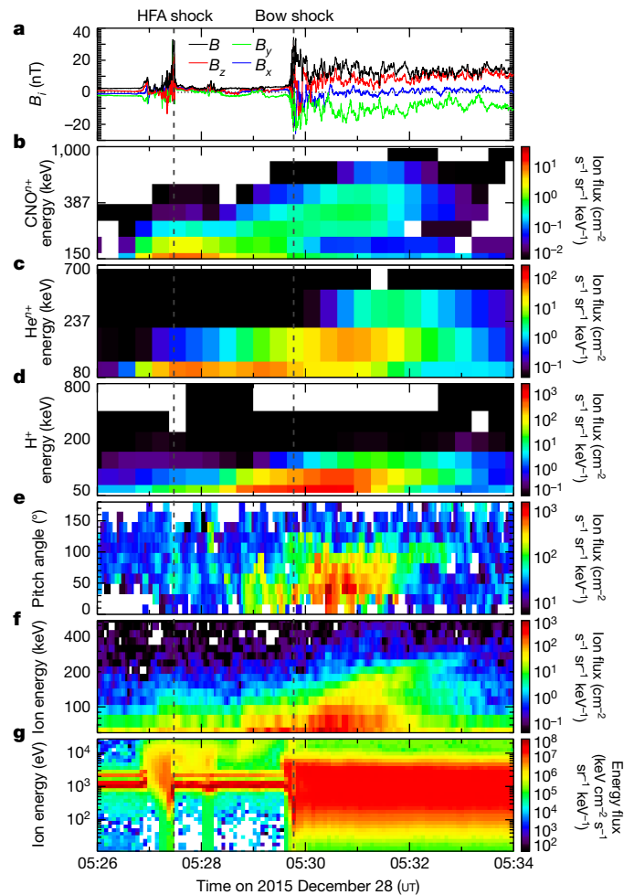
Fig. 2 | MMS observations of energetic ions and context data during and after the encounter with the HFA. b–d, Heavy-ion ( \text{CNO}^{m+} ; b), helium ( \text{He}^{m+} ; c) and proton ( \text{H}^+ ; d) data from the energetic particle detector EIS (EPD/EIS). The colour scales show the differential fluxes and the energies shown (on the y axes) are the total energy per incident ion. e, Pitch angle distributions for 70–105-keV ions from the EPD/FEEPS instruments. For b–e, the data were compiled from counts on the EIS or FEEPS instruments on all four spacecraft. f, g, Total ion energy distributions from all four FEEPS instruments (f) and the DIS instrument on MMS-3 (g). a, Magnetic-field vector components and strength from MMS-3, for context. The grey, dashed, vertical lines mark the HFA shock and the bow shock, as labelled. The energetic ions were first observed within the HFA around 05:27 UT and then continuously after the HFA through the ion foreshock and into the magnetosheath until around 05:33 UT.
