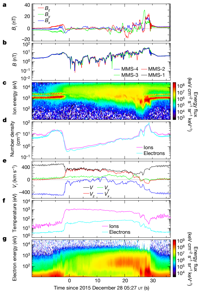
Fig. 1 | Overview of the MMS burst data during the HFA. a–g. Quantities shown (all from MMS-1 unless otherwise specified) are the components of the magnetic-field vector \mathbf{B} = (B_x, B_y, B_z) (a) and the magnetic-field strength B = |\mathbf{B}| from the flux-gate magnetometers on each of the four spacecraft (b); the omni-directional, averaged energy distributions of the ions from the fast plasma investigation dual ion spectrometer (FPI/DIS) (c); the ion and electron densities (d); the components of the velocity vector of the ions ( V_x, V_y, V_z ) and its magnitude V = |\mathbf{V}| (e); the ion and electron temperatures (f); and the omni-directional, averaged energy distributions of the electrons from the FPI dual electron spectrometer (FPI/DES) (g). With the geometry and multipoint observations of the HFA, its size, expansion rate and motion along the bow shock can be calculated. Using the rotation of the IMF before and after the HFA, we estimate the normal direction of the IMF discontinuity that is responsible for the formation of the HFA to be \mathbf{n} = (0.70, -0.44, -0.57) in the geocentric solar ecliptic coordinate system. We calculated the normal direction of the upstream shock of the HFA using co-planarity and multi-spacecraft analysis (Methods), yielding \mathbf{n}_{sh} = (0.85, -0.16, -0.53) and \mathbf{n}_{sh} = (0.84, -0.44, -0.31) , respectively, which are generally consistent. In the solar-wind frame, the HFA shock was expanding upstream (towards the Sun) at about 360 \text{ km s}^{-1} . When MMS observed the HFA, it was expanding at a rate of 108 \text{ km s}^{-1} along the IMF discontinuity normal and was approximately 16,000 \text{ km} (2.5 Earth radii) in size from edge to edge along the track taken by MMS through the HFA. The geometry of the HFA and the values that we have calculated are critical for enabling comparisons between observed particle acceleration signatures and theory.
