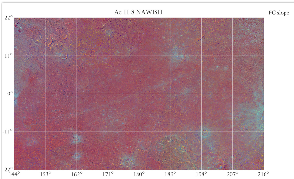
Fig. 2. RGB composite map of the Ac-H-8 Nawish quadrangle made from FC color ratios: F5/F3 (965 nm/749 nm), F2/F3 (555 nm/749 nm), and F8/F3 (438 nm/749 nm). Color ratios may enhance differences in material and composition. (For interpretation of the references to colour in this figure legend, the reader is referred to the web version of this article.)
