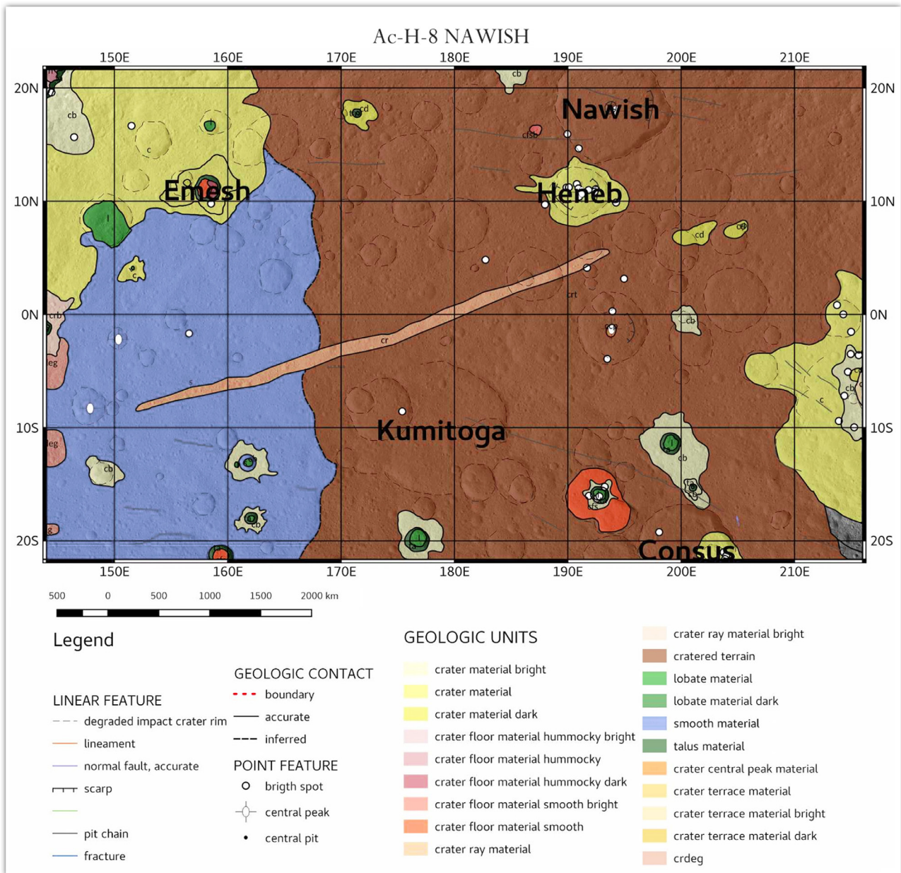
Fig. 4. Geological map of Ac-H-8 Nawish quadrangle, from Frigeri et al. (2018b). The broad brownish geologic unit is mapped as ‘cratered terrain’ (crt). Yellow patches represent ‘crater material’, (c) while blue unit indicates ‘smooth material’ (sm).
