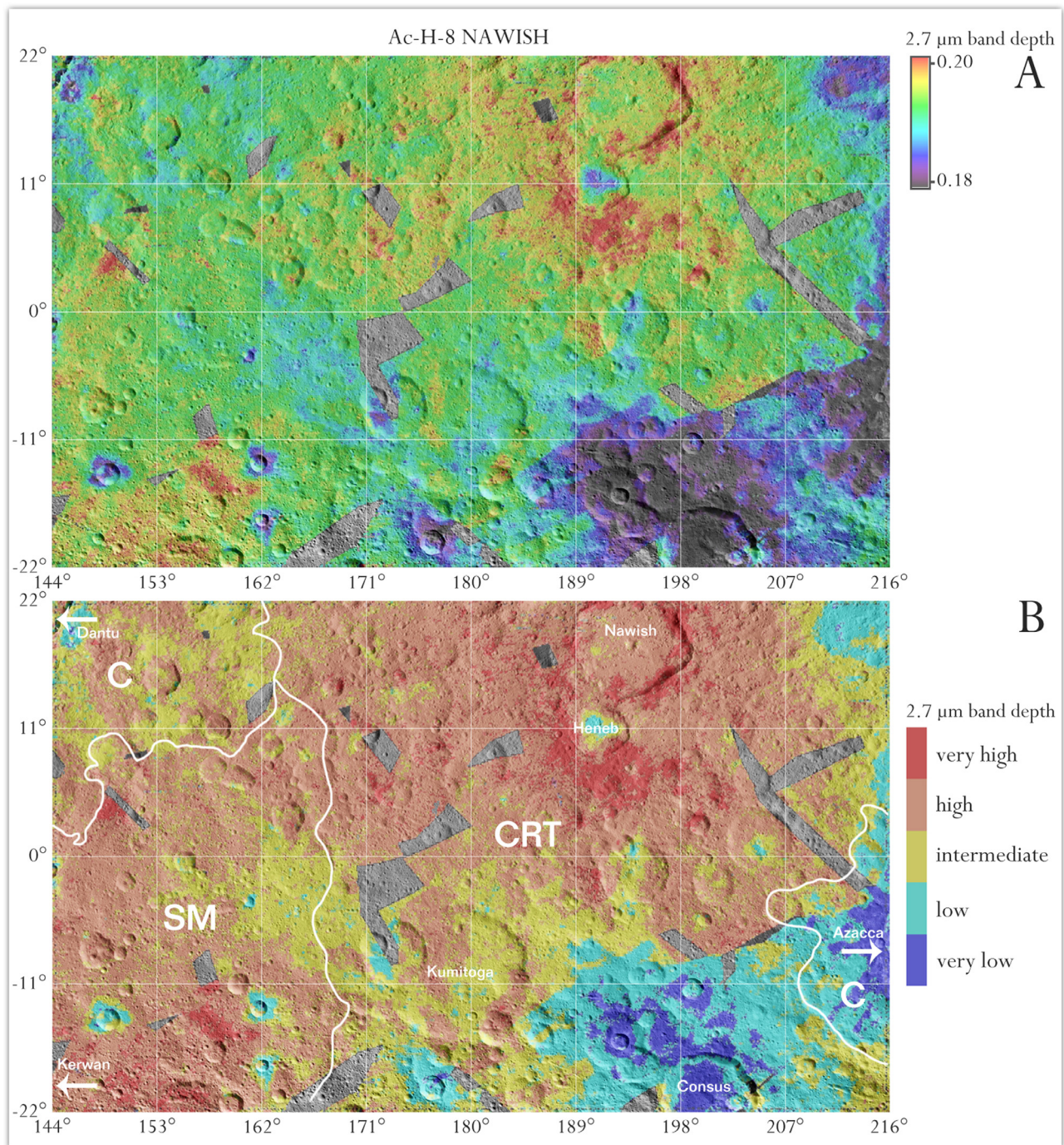
Fig. 7. (A) 2.7 \mu\text{m} band depth VIR-derived map of the Nawish quadrangle. (B) The map shown in Panel A divided in 5 different ranges of values to emphasize its relationship with the geological units. The boundary of some geological units has been drawn (white curves: CRT = cratered terrains, C = crater material, SM = smoothed material, for details see Frigeri et al., 2018b). The map is superimposed over the FC images using a transparency of 25%.
