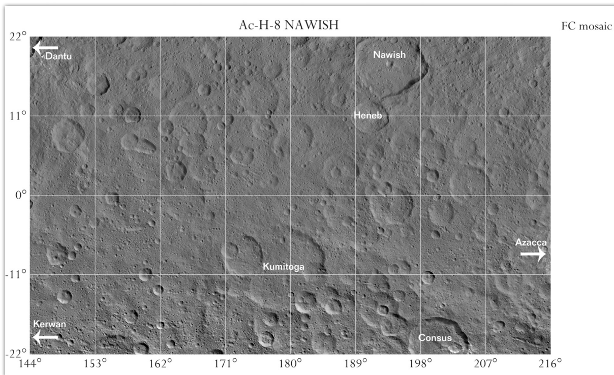
Fig. 1. Reflectance map of Ac-H-8 Nawish, obtained through photometric correction of FC clear-filter data acquired in the HAMO mission phase. The map scale is ~ 140 m/pixel.
