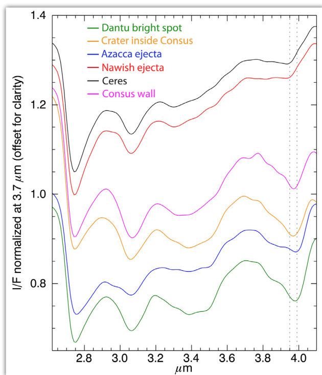
Fig. 10. Average spectra of different regions on Ceres surface compared with some areas of interest in Ac-H-8 Nawish quadrangle. The spectra have been normalized to 1 at 3.7 \mu\text{m} . An offset has been applied for clarity. The spectra are an average of 10 pixels. Dotted lines show the shift of the band center at 4 \mu\text{m} , indicating a compositional variation of carbonate species.
