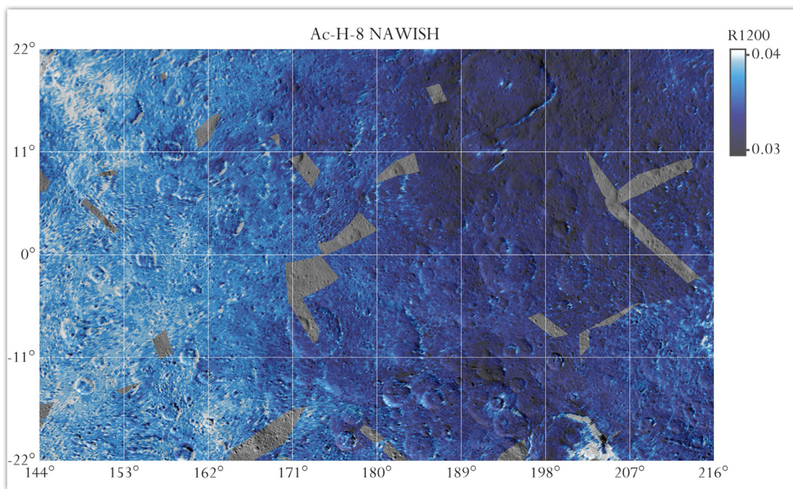
Fig. 5. Reflectance map of Ac-H-8 Nawish, obtained through photometric correction of VIR data acquired at 1.2 \mu\text{m} in the HAMO mission phase, interpolated on a grid with a fixed resolution of 140 m/pixel, photometrically corrected by using the method described by Ciarniello et al. (2017), i.e. a Hapke photometric correction to standard observation geometry ( i = 30^\circ , e = 0^\circ , \alpha = 30^\circ ). The map is superimposed over the Framing Camera (FC) images using a transparency of 25%.
