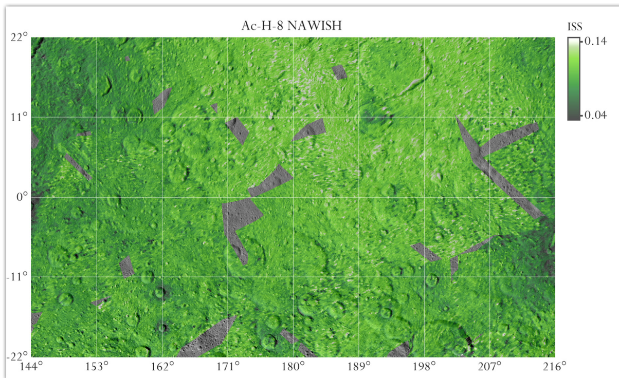
Fig. 6. VIR spectral slopes calculated in the near infrared range 1.163–1.891 \mu\text{m} (ISS). The map is superimposed over the FC images using a transparency of 25%.
