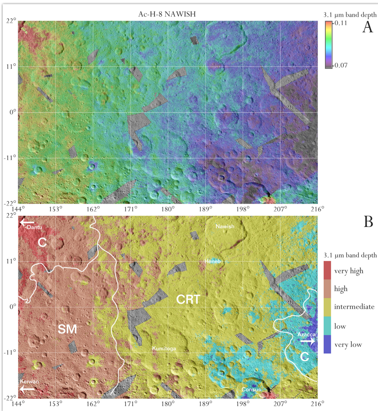
Fig. 8. (A) 3.1 μm band depth VIR-derived map of the Nawish quadrangle. (B) The map shown in Panel A divided in 5 different ranges of values to emphasize its relationship with the geological units. The boundary of some geological units has been drawn (white curves: CRT = cratered terrains, C = crater material, SM = smoothed material, for details see Frigeri et al., 2018b). The map is superimposed over the FC images using a transparency of 25%.
