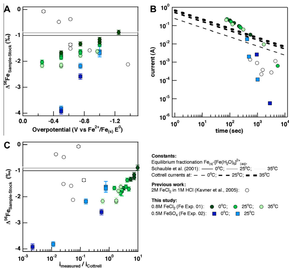
Fig. 4. Results from iron experiments showing: (A) \Delta^{56}\text{Fe} vs. overpotential; (B) effect of temperature on the diffusion-limiting Cottrell current calculated for 0.78 M stock solution of iron (dashed lines) with experimental current superimposed; (C) \Delta^{56}\text{Fe} vs. the ratio of experimental current to Cottrell diffusion-limiting current.
