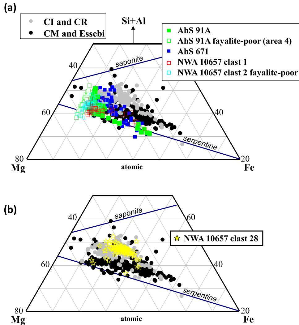
Figure 2. Shown are (Si+Al)–Mg–Fe atomic percent ternary diagrams plotting compositions of phyllosilicates in AhS 91A, AhS 671, and three CC-like xenoliths in polymict ureilite NWA 10657 compared with those in CI, CR, and CM carbonaceous chondrites. Lines represent observed stoichiometric compositions of serpentine and saponite solid solution series (Deer et al. 1962; Fleet 2003). Data for xenoliths were obtained by line scans of broad-beam analyses of matrix areas and then filtered to remove analyses with high FeO (presumably including magnetite and/or fayalite and/or sulfides) and CaO (including Ca-rich phases), as well as those with extremely low totals. Data for AhS 91A, AhS 671, and CC are from Goodrich et al. (2019a).
