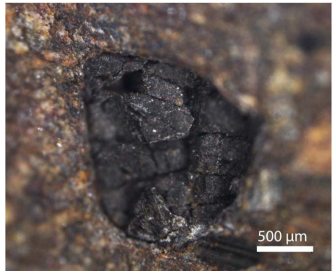
Figure A1. Clast 28 of NWA 10657 on the surface of the slab. Optical photomicrograph.
