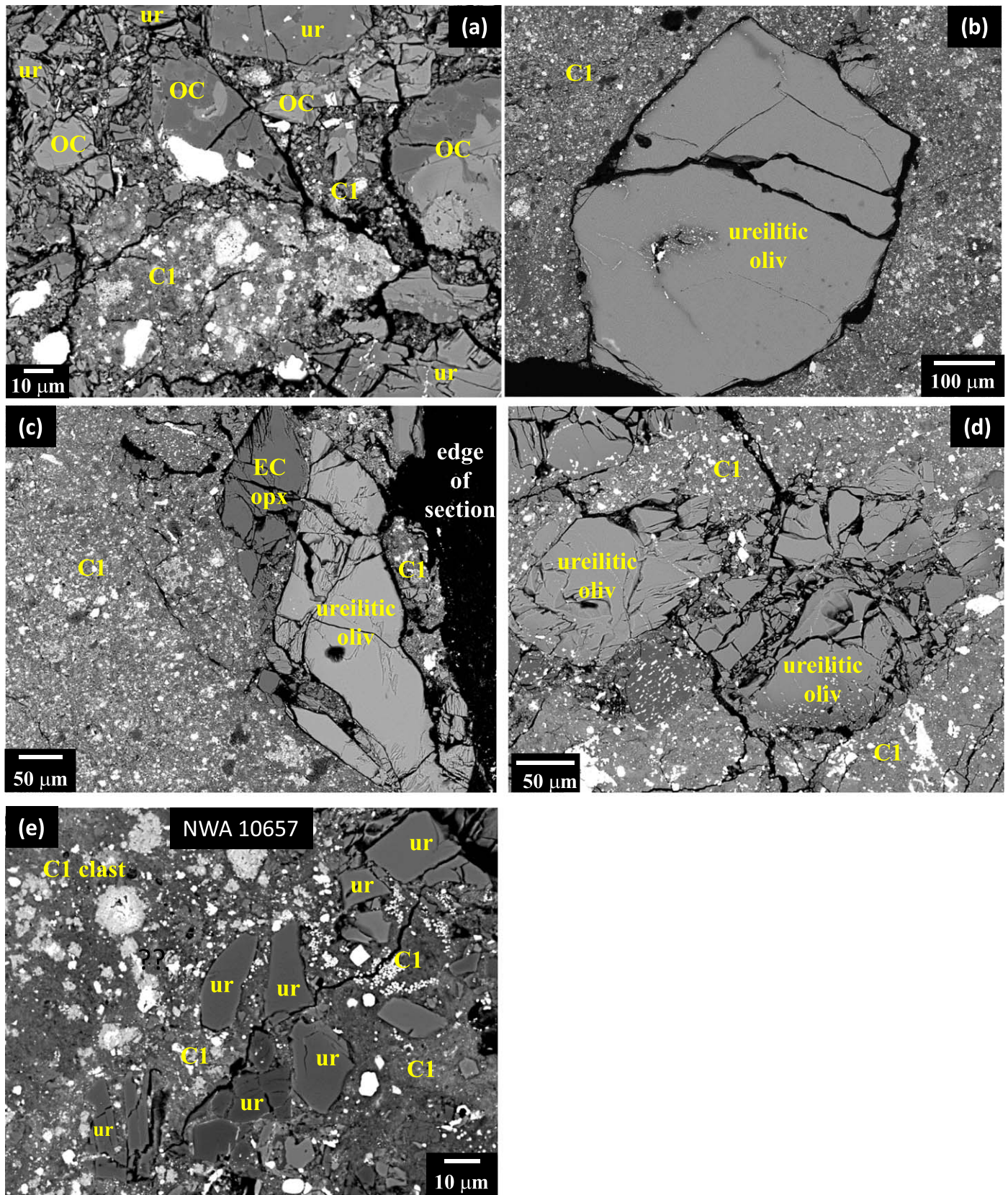
Figure 7. BEIs showing textures of CC-like (C1) lithologies in polymict ureilites in contact with ureilitic (ur), OC, and EC components of their host breccias in polymict ureilites. (a)–(d) AhS 91A or AhS 671. (e) NWA 10657 clast 2, brecciated boundary with surrounding ureilitic materials. opx = orthopyroxene; oliv = olivine.
